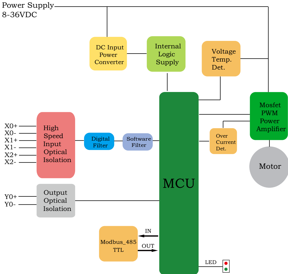
IG35ET Block Diagram
